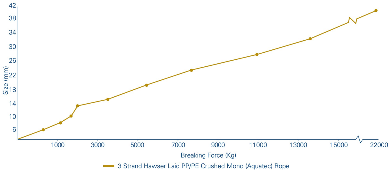
Breaking Force Graph
